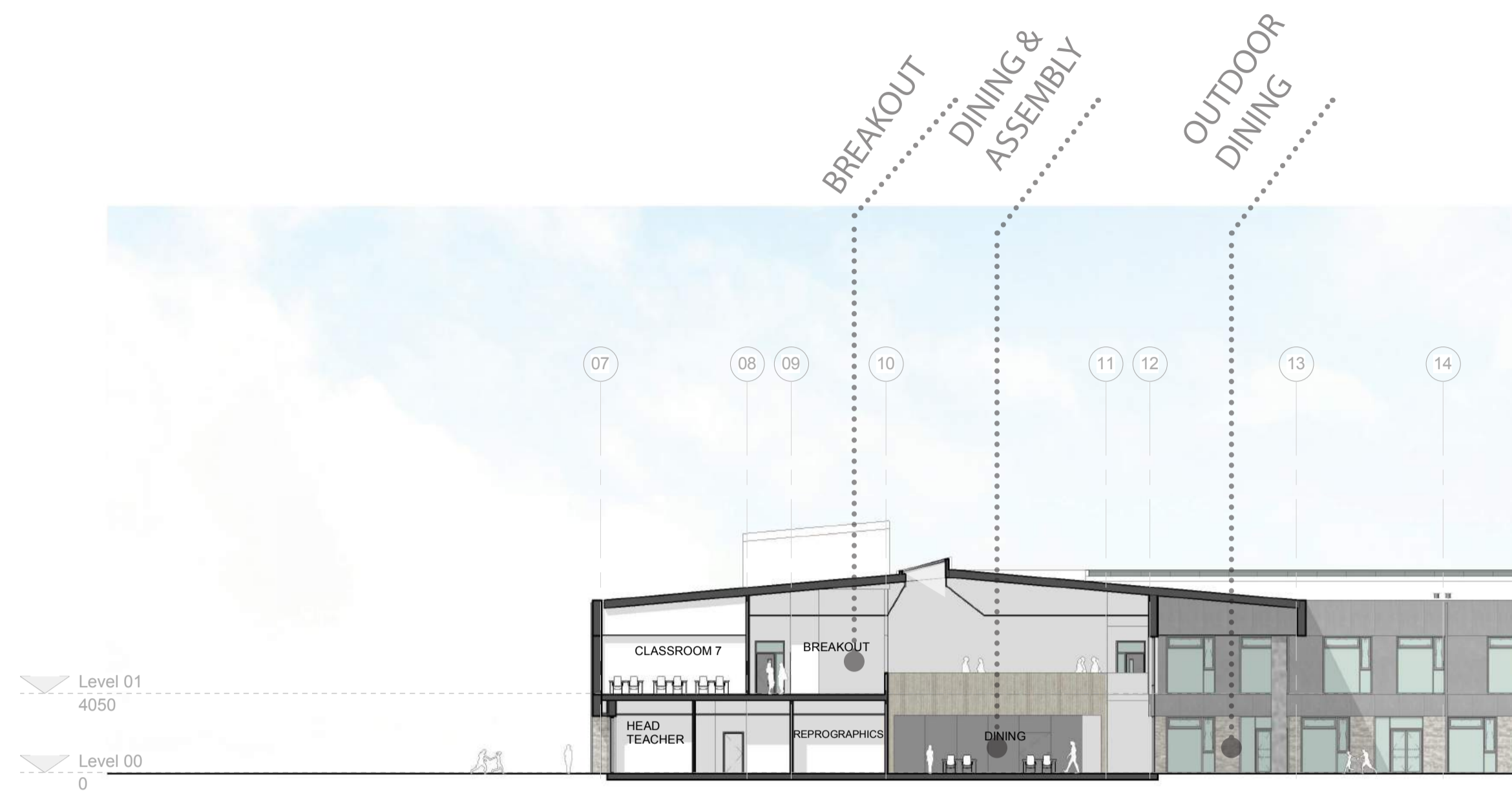
SECTION B-B
