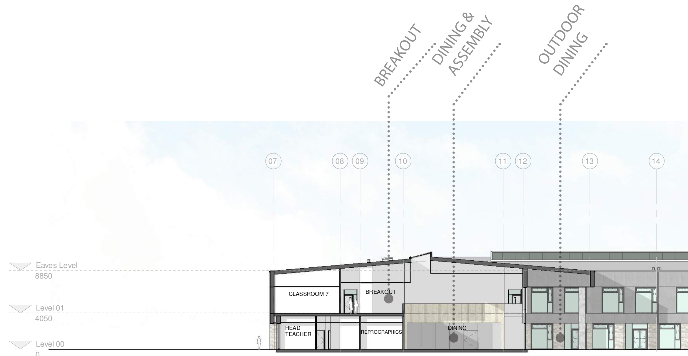
SECTION B-B
