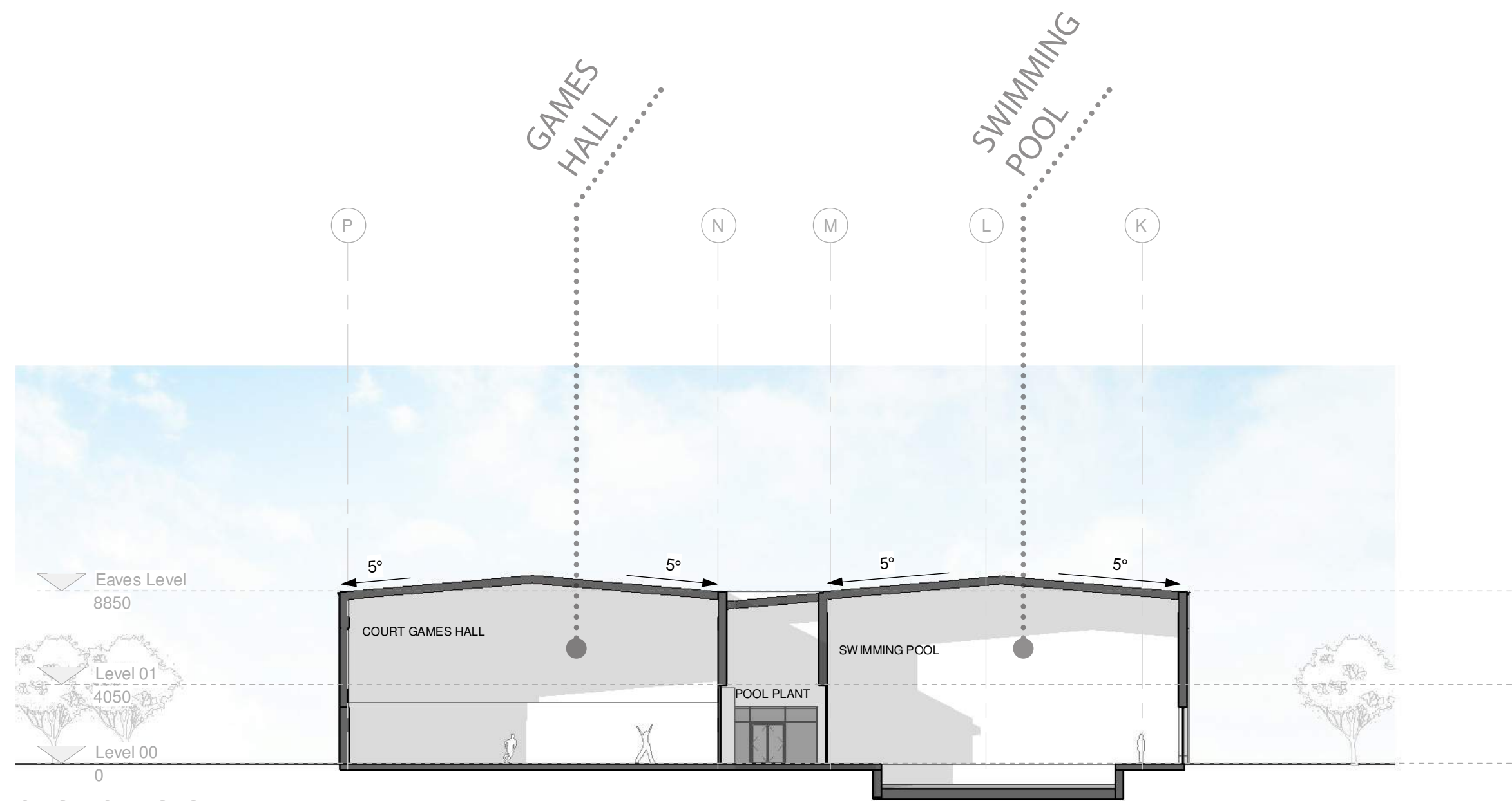
SECTION C-C
