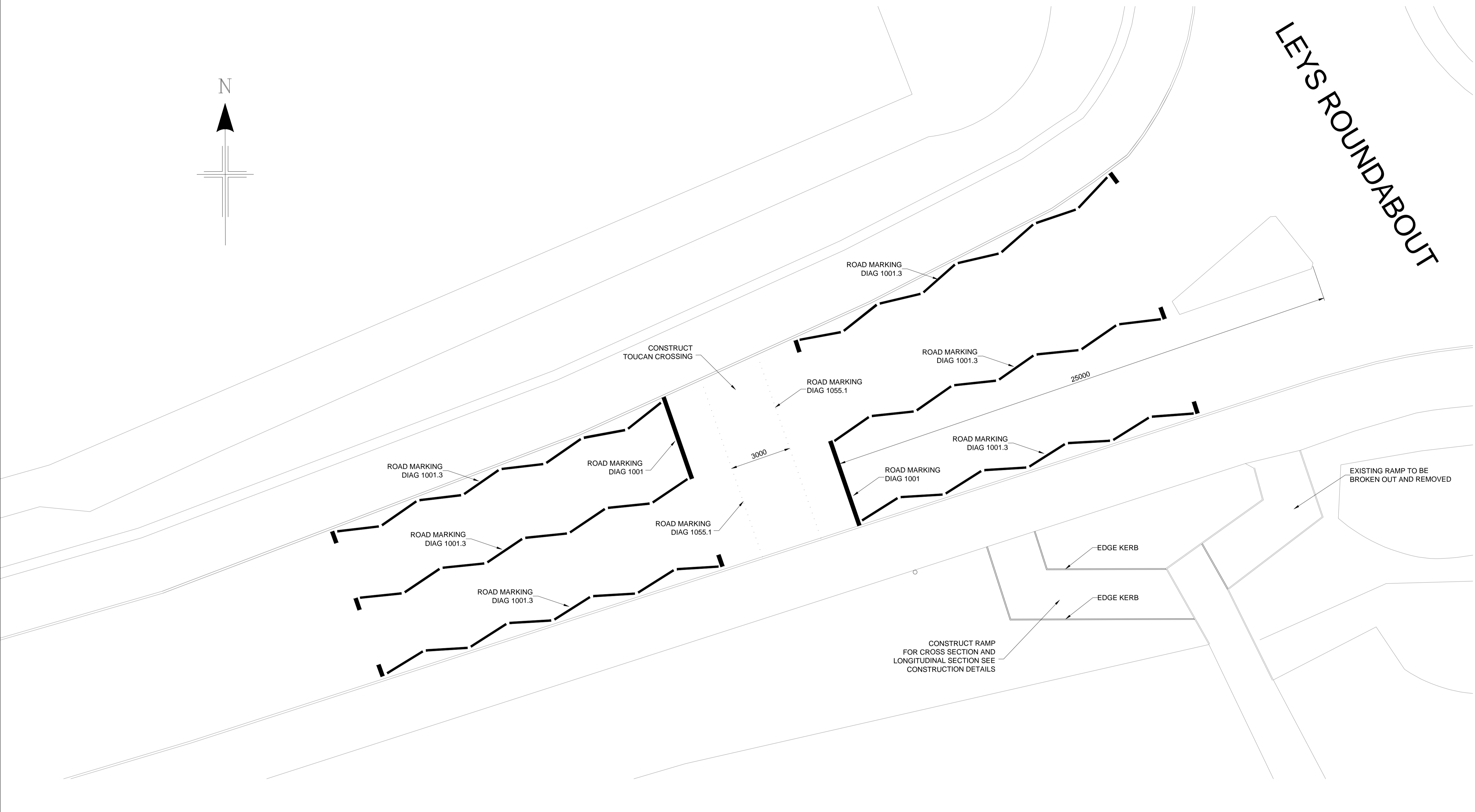
TOUCAN CROSSING B8082 LEYS ROUNDABOUT Scale 1:100
