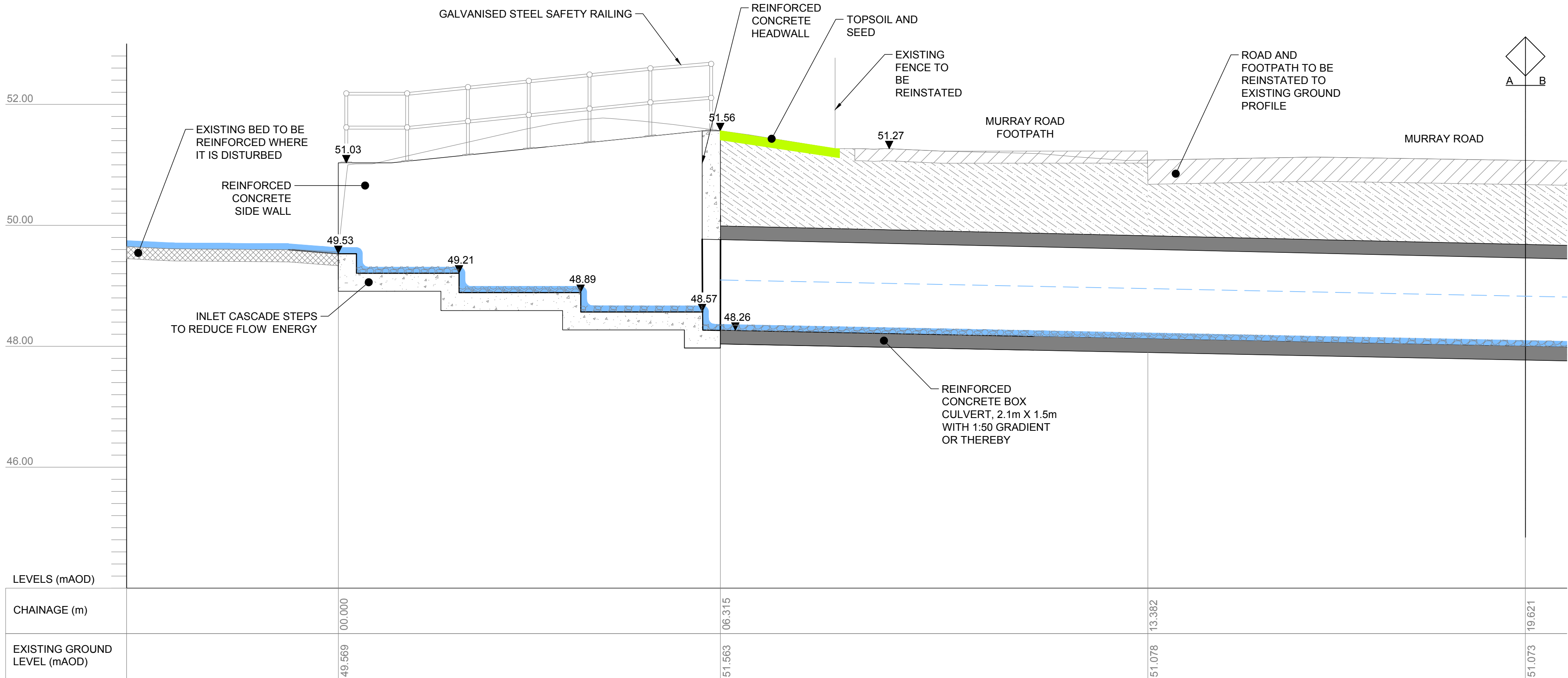
SECTION 1-1 (SP-04)
