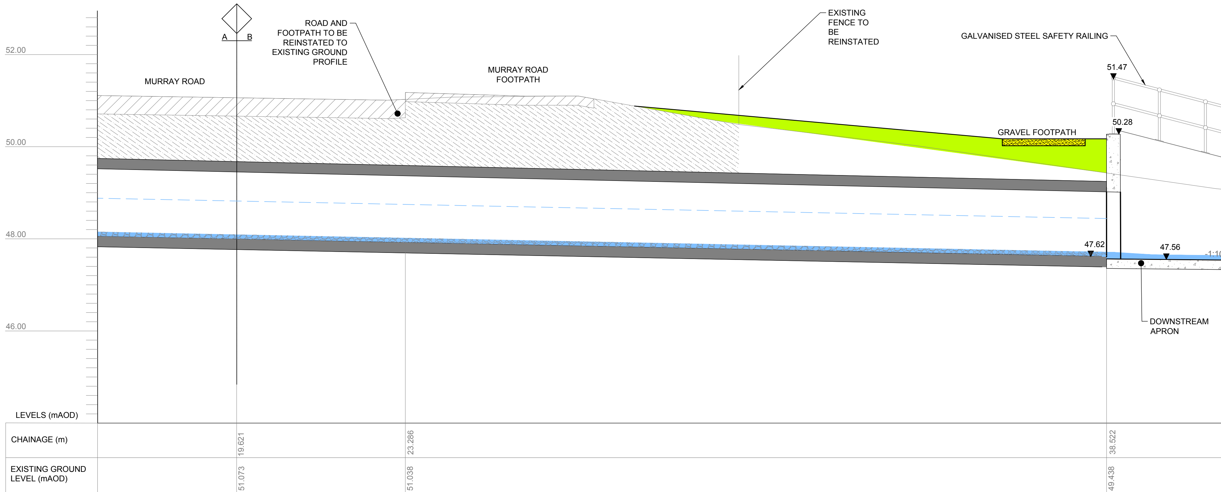
SECTION 1-1 (SP-04)
