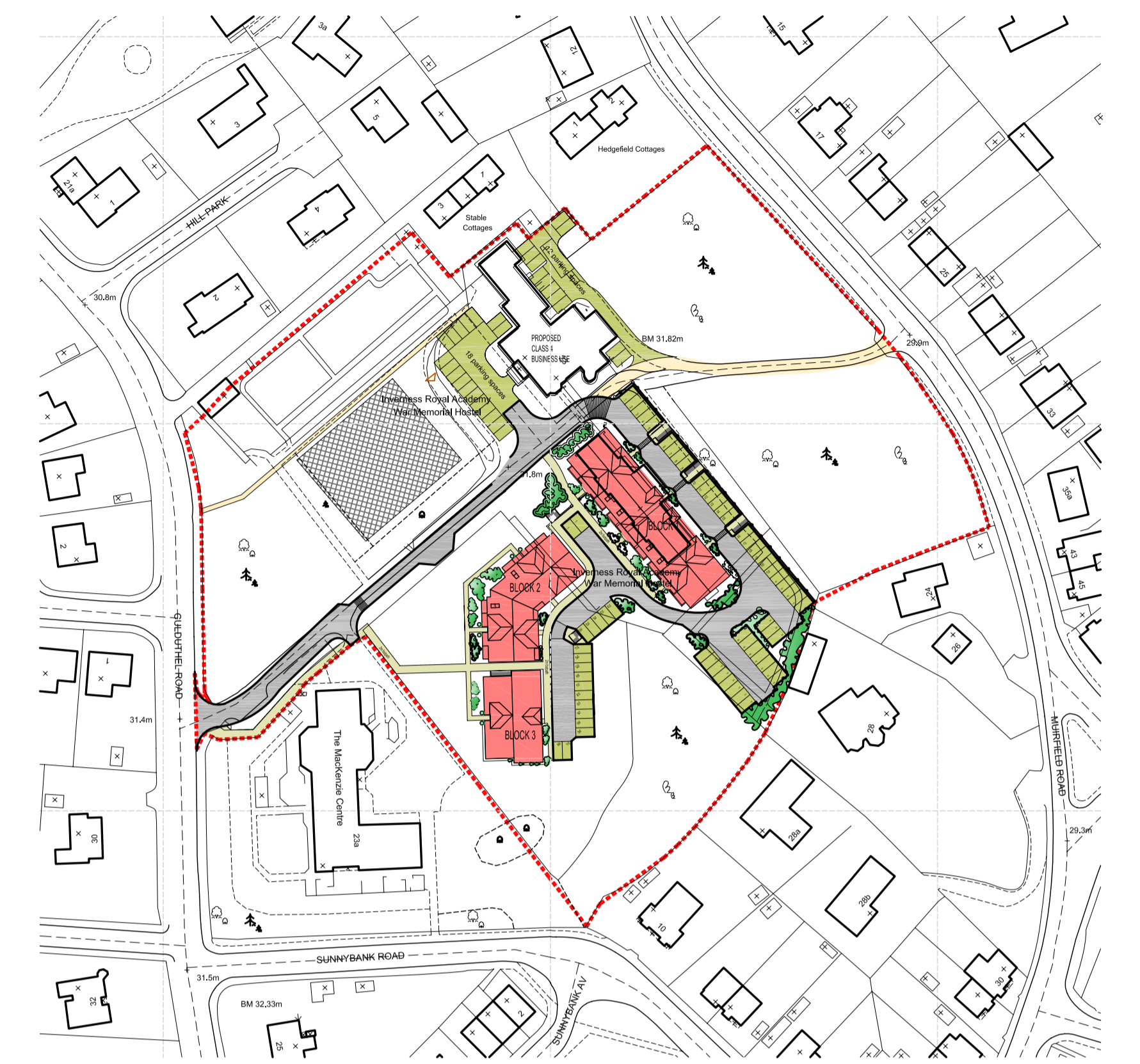
LOCATION PLAN
