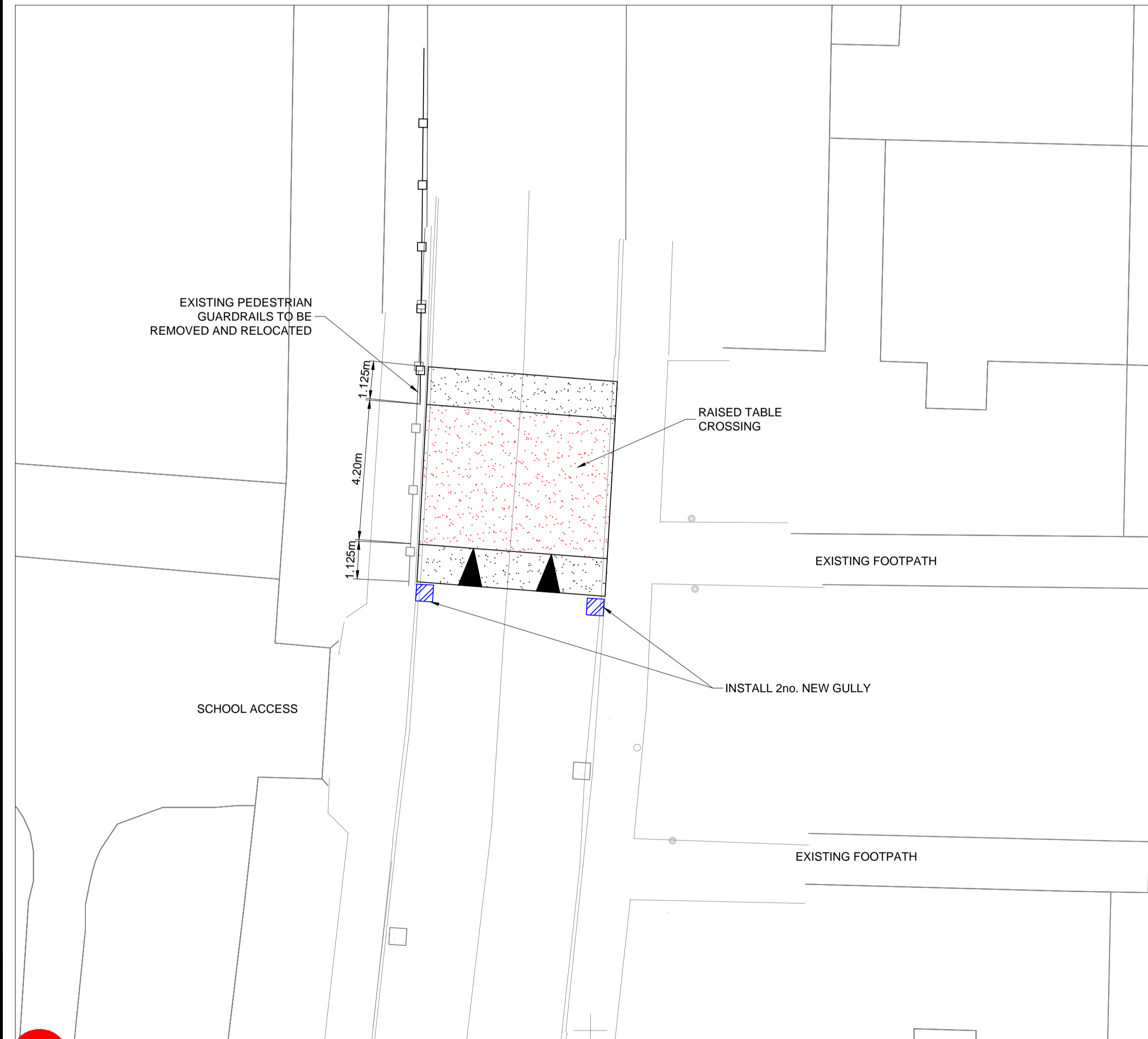
AREA 01 SCALE 1:100
