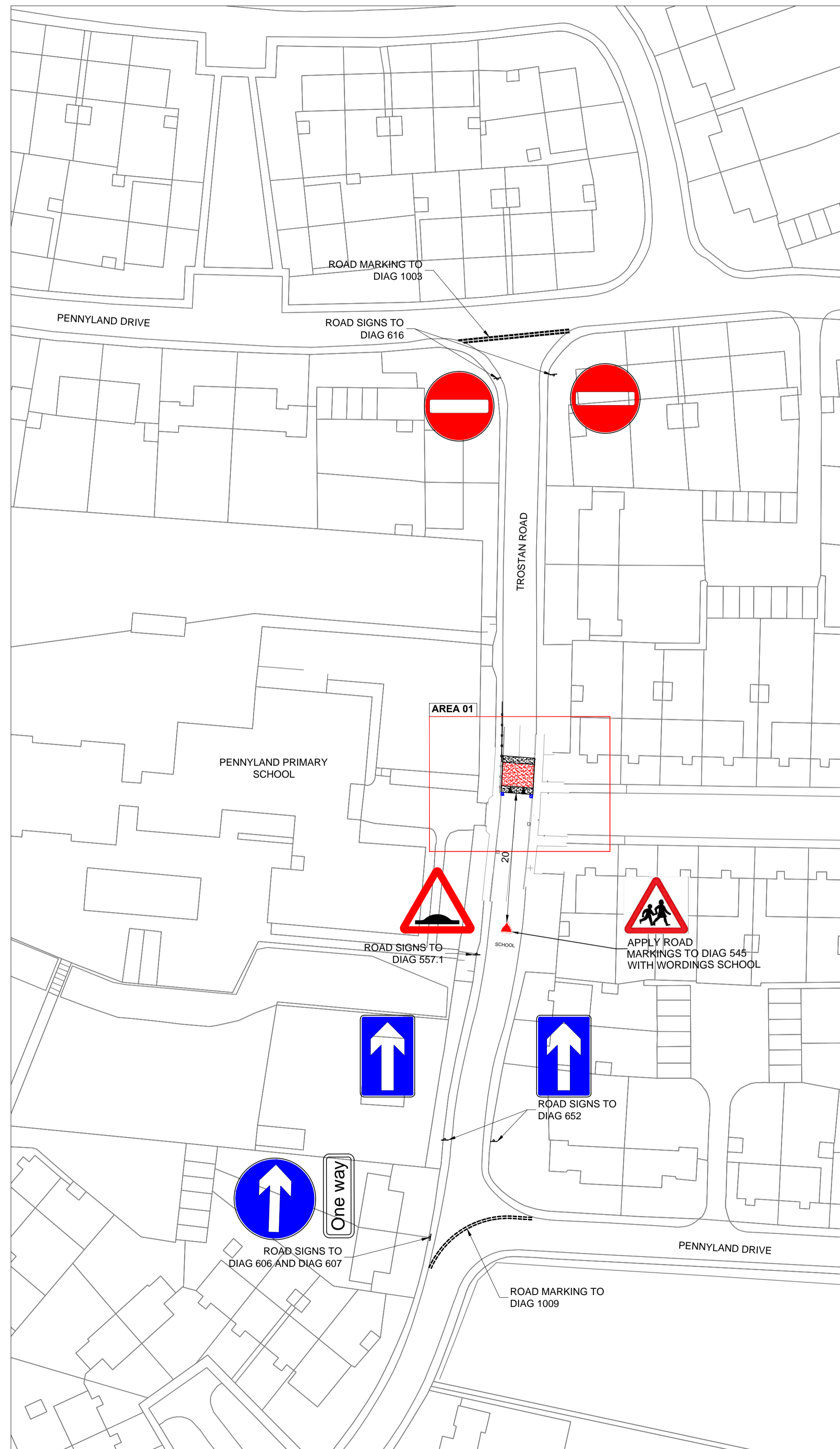
GENERAL LAYOUT SCALE 1:500
