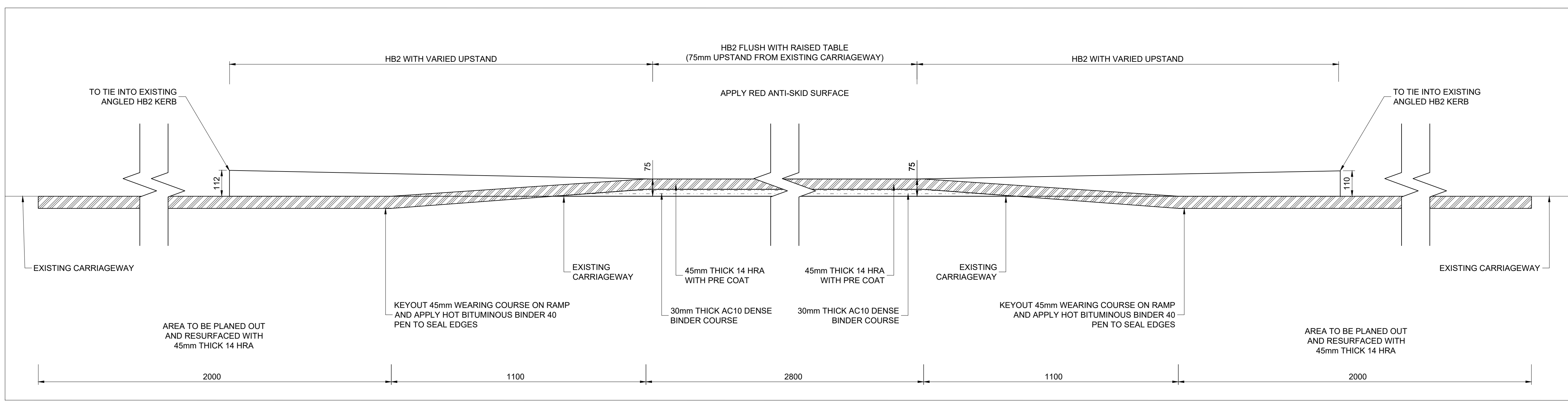
DETAIL 02 SCALE 1:10
