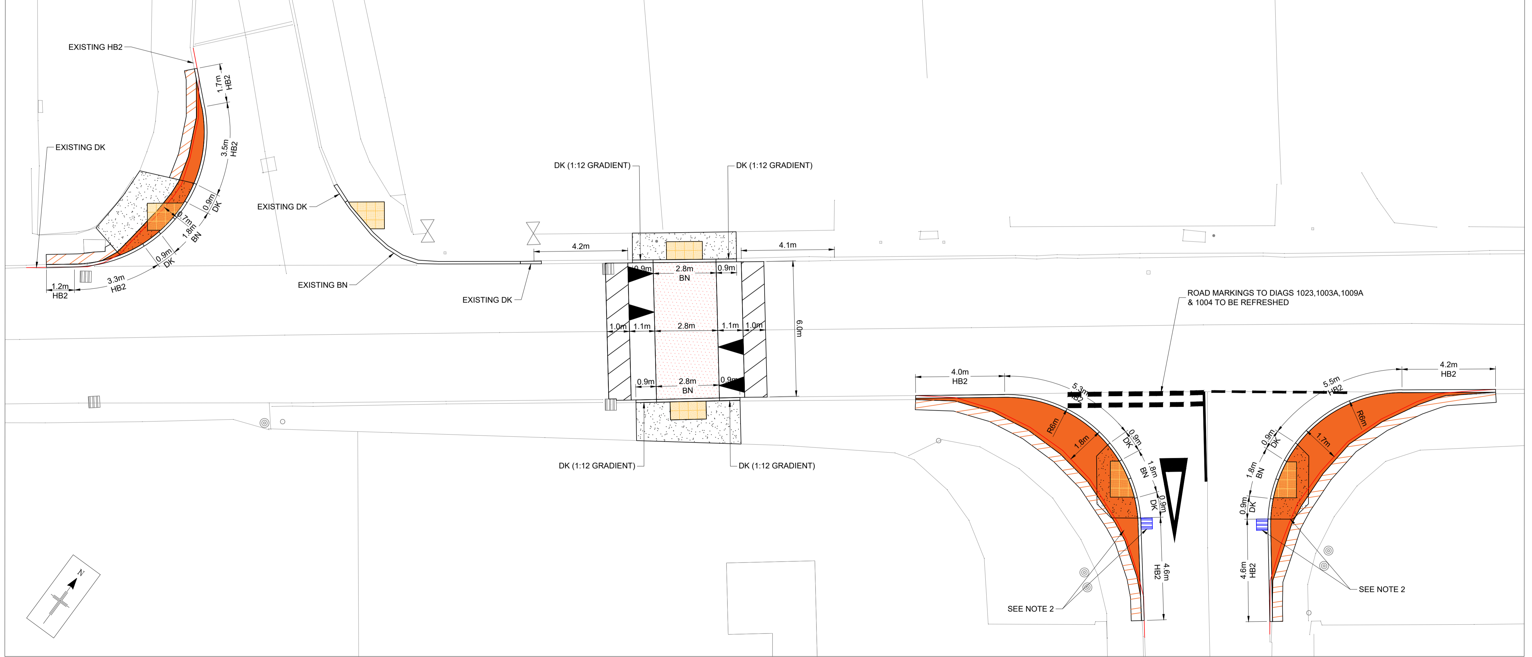
DETAIL 01 SCALE 1:100
