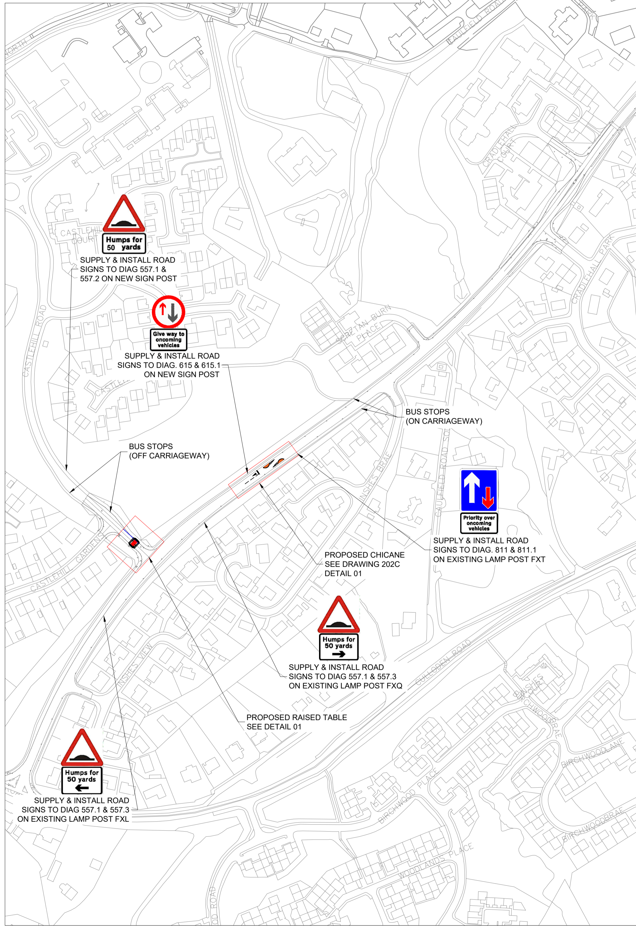
GENERAL LAYOUT SCALE 1:2000
