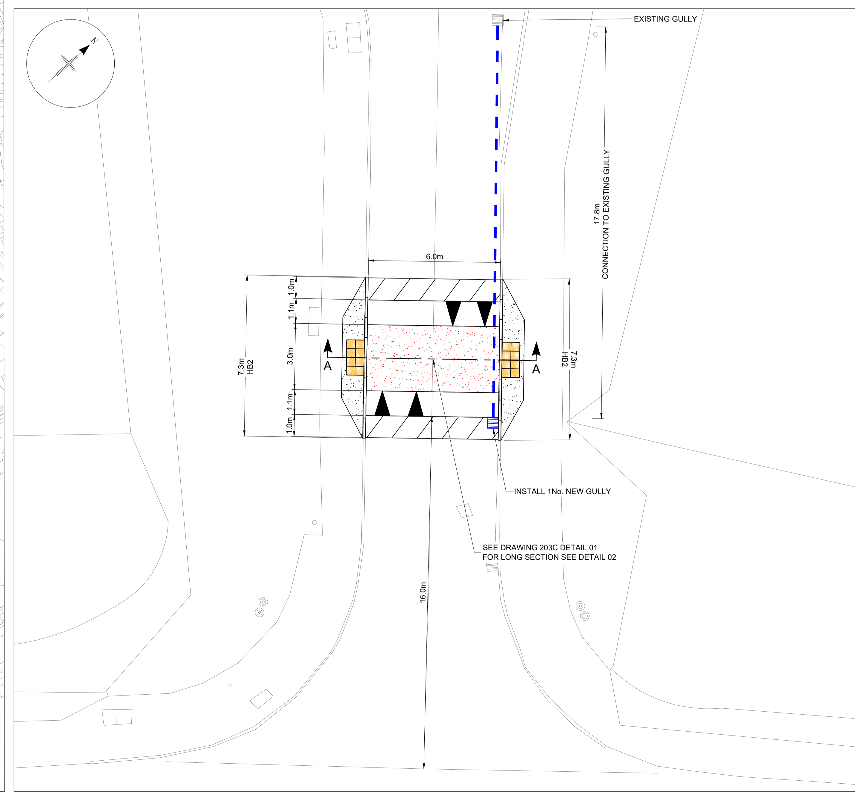
DETAIL 01 SCALE 1:100
