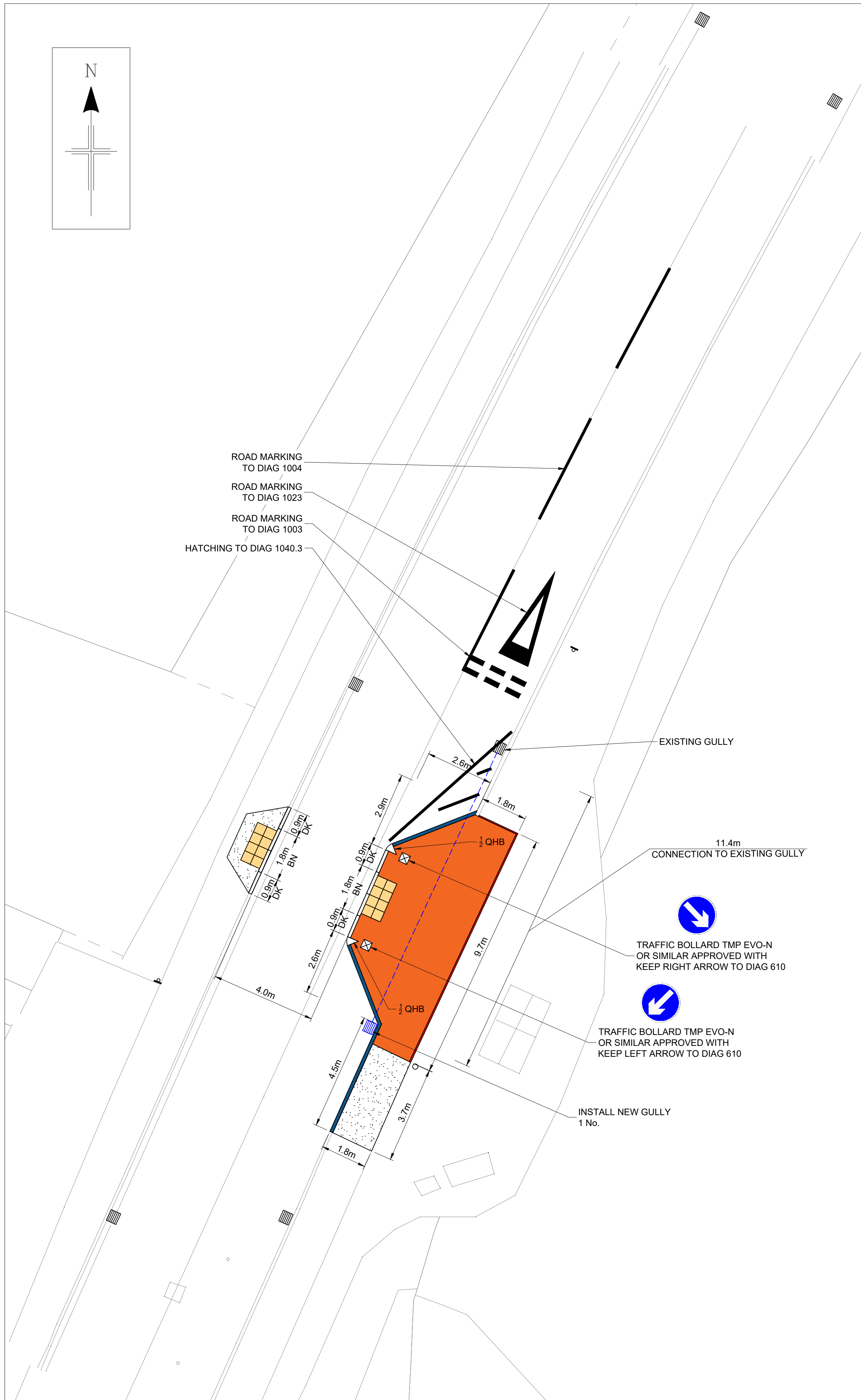
DETAIL 01 SCALE 1:100
