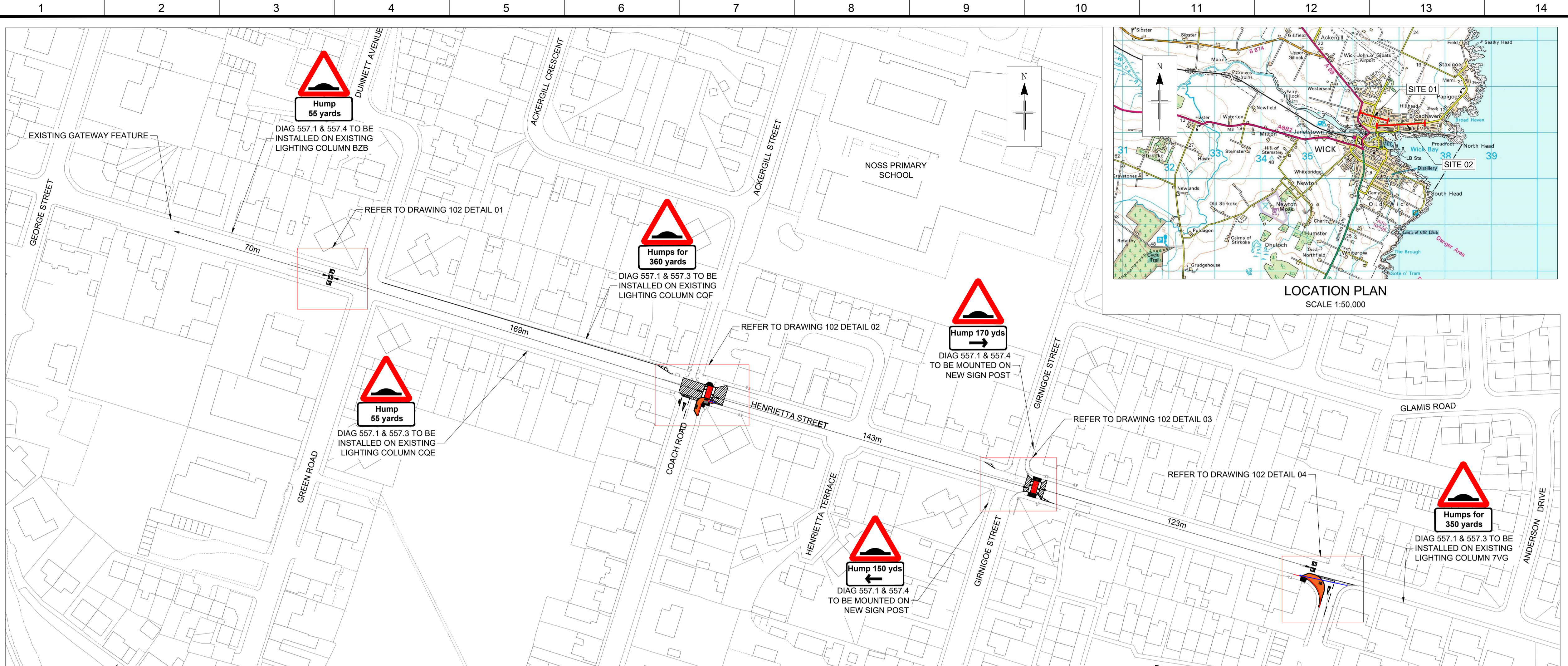
GENERAL LAYOUT - HENRIETTA STREET SCALE 1:1000
