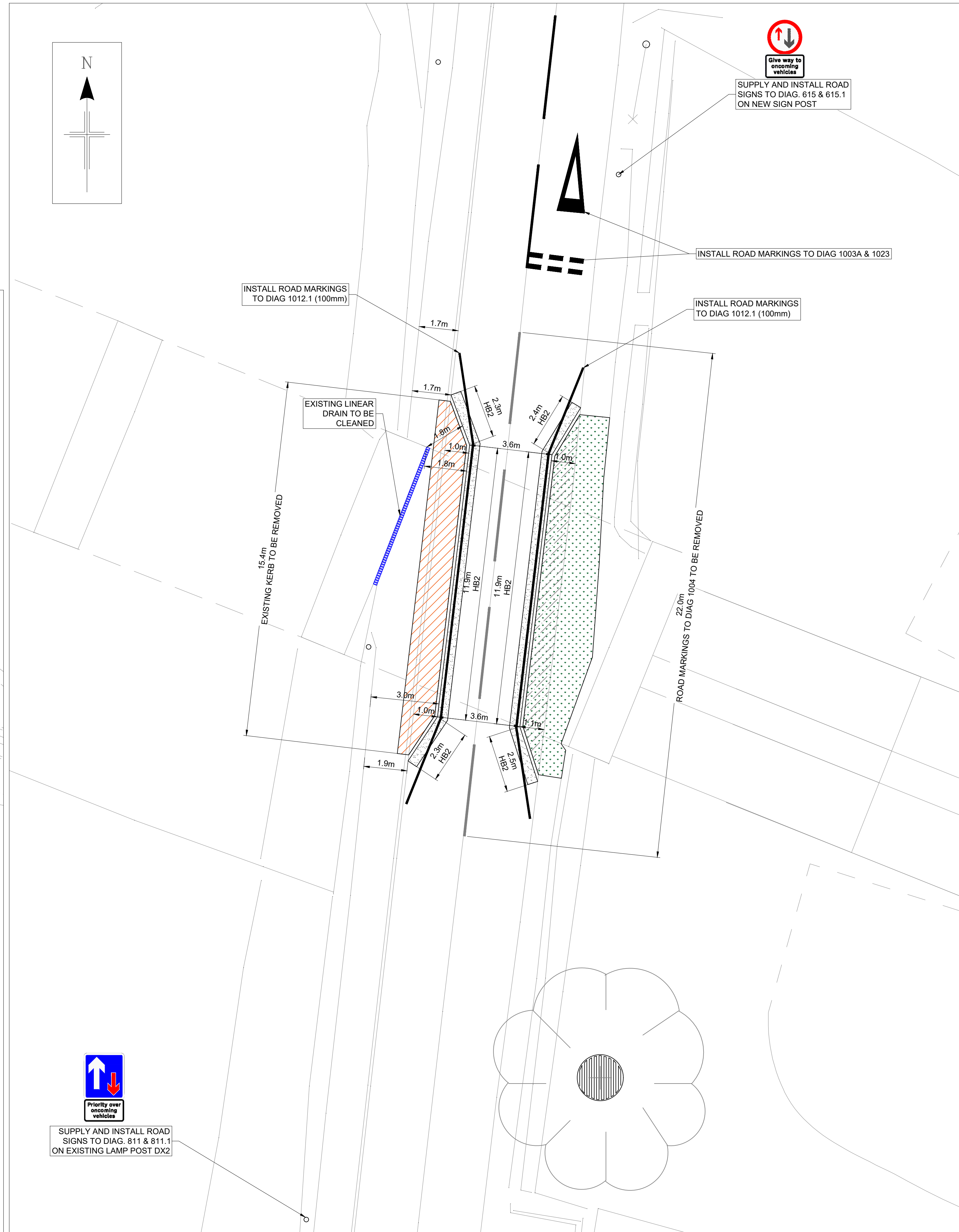
DETAIL 01 SCALE 1:100
