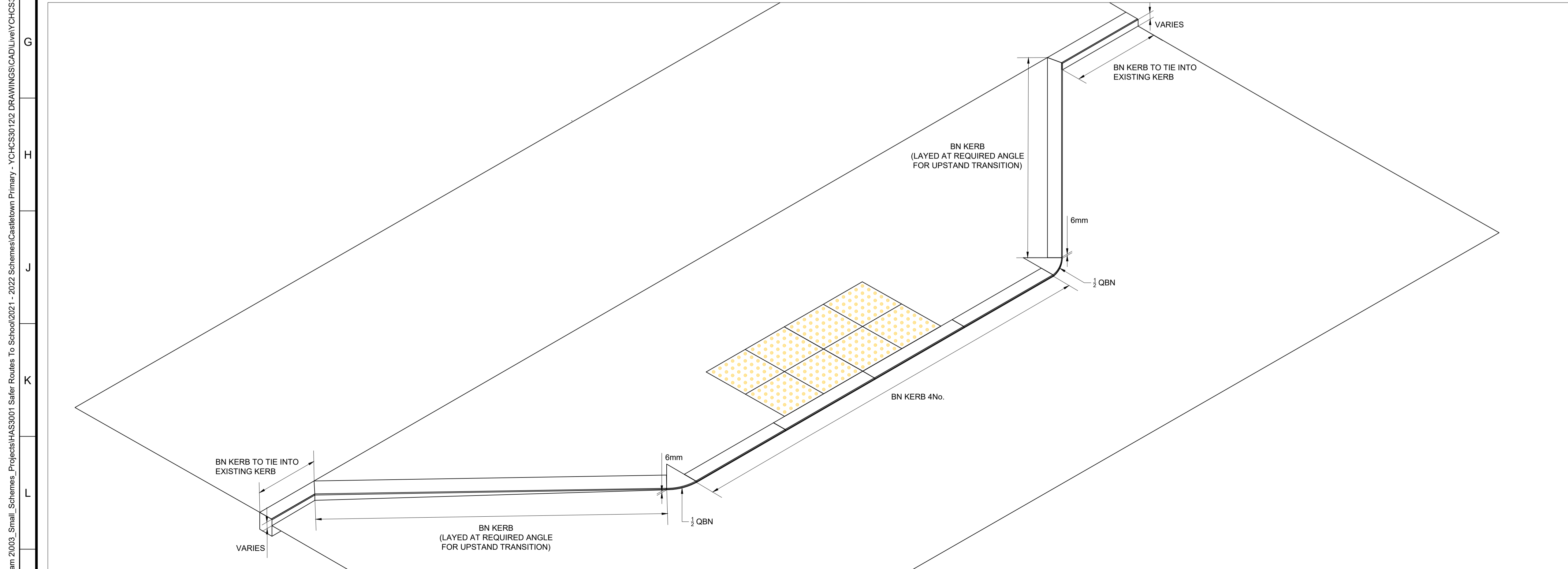
DETAIL 02- ISOMETRIC VIEW OF GENERAL KERB ARRANGEMENT SCALE 1:20
