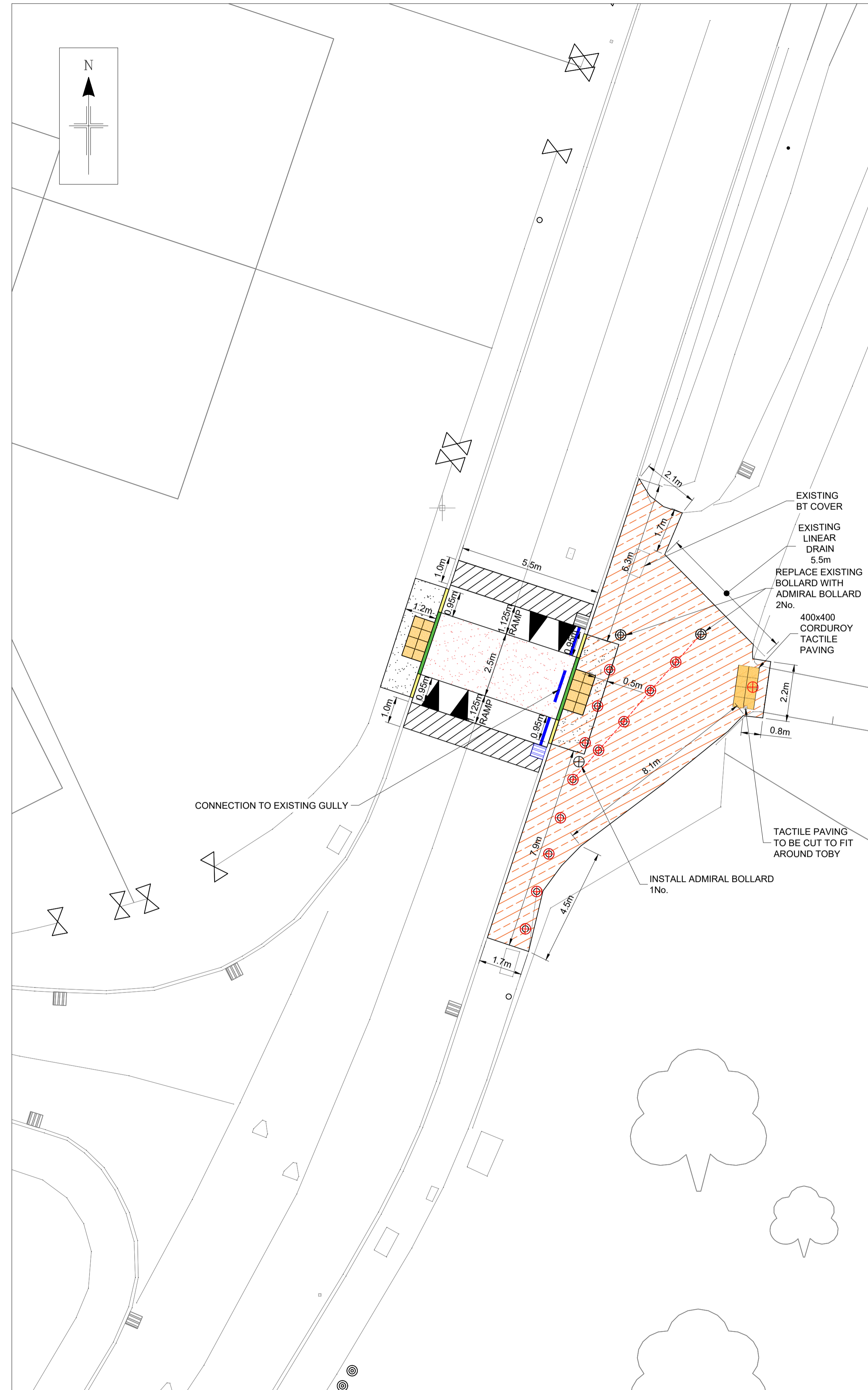
DETAIL 01 SCALE 1:100
