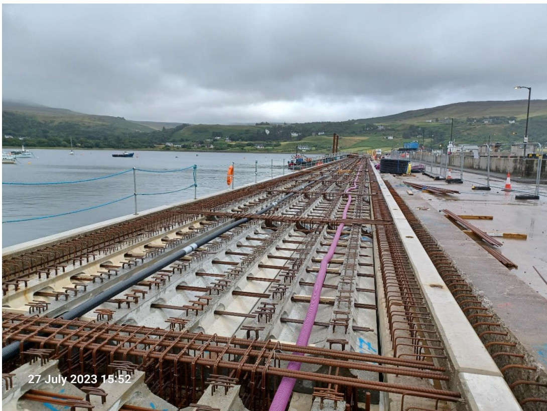
Approachway Widening – Installation of Precast and Concrete
