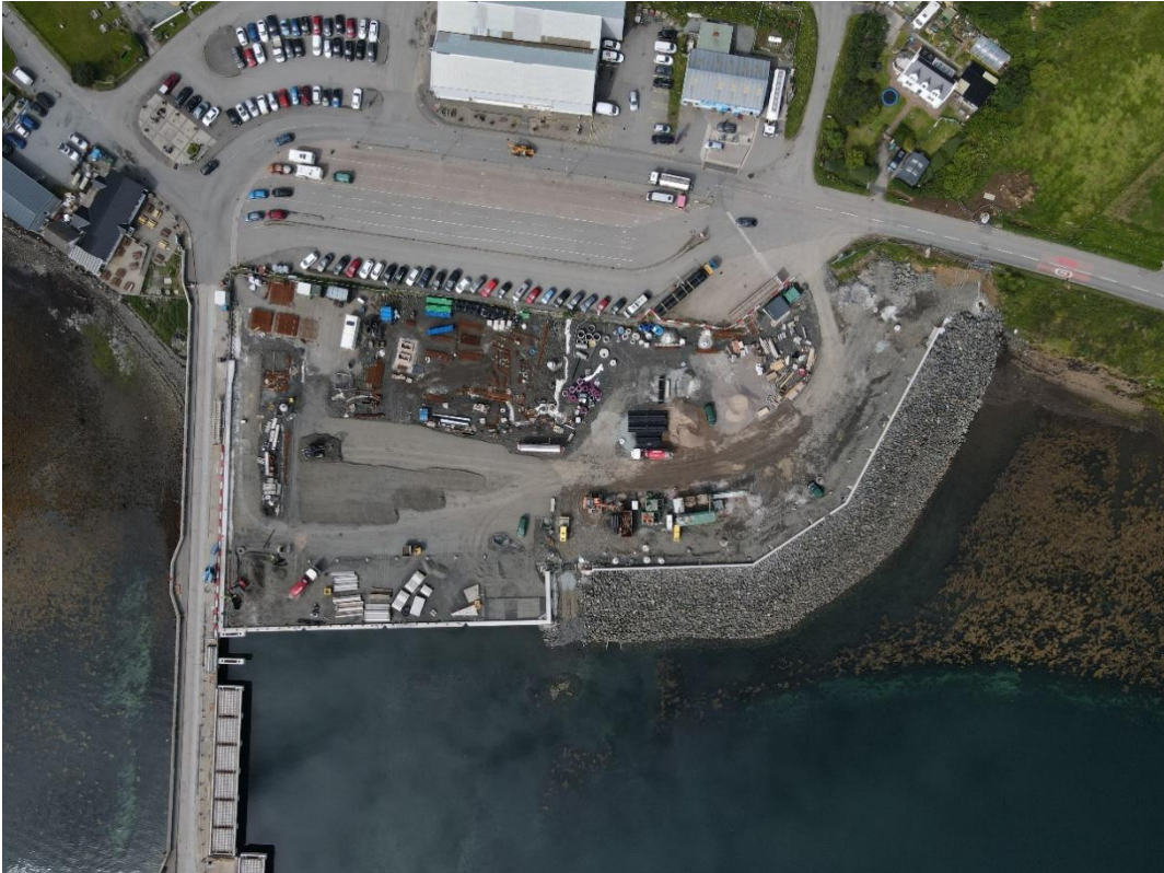
Marshalling Area Reclamation
