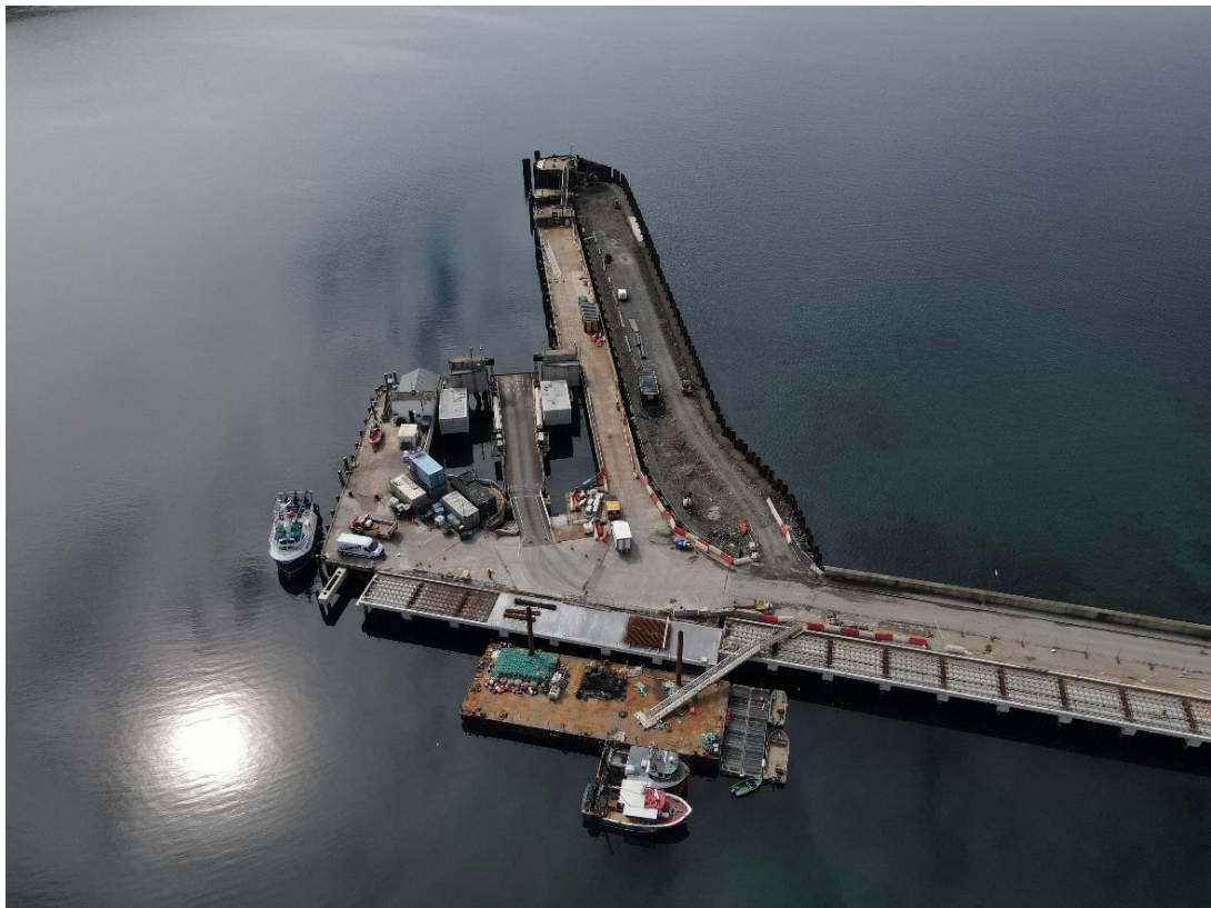
Berthing Structure Widening and Roundhead – Infill
