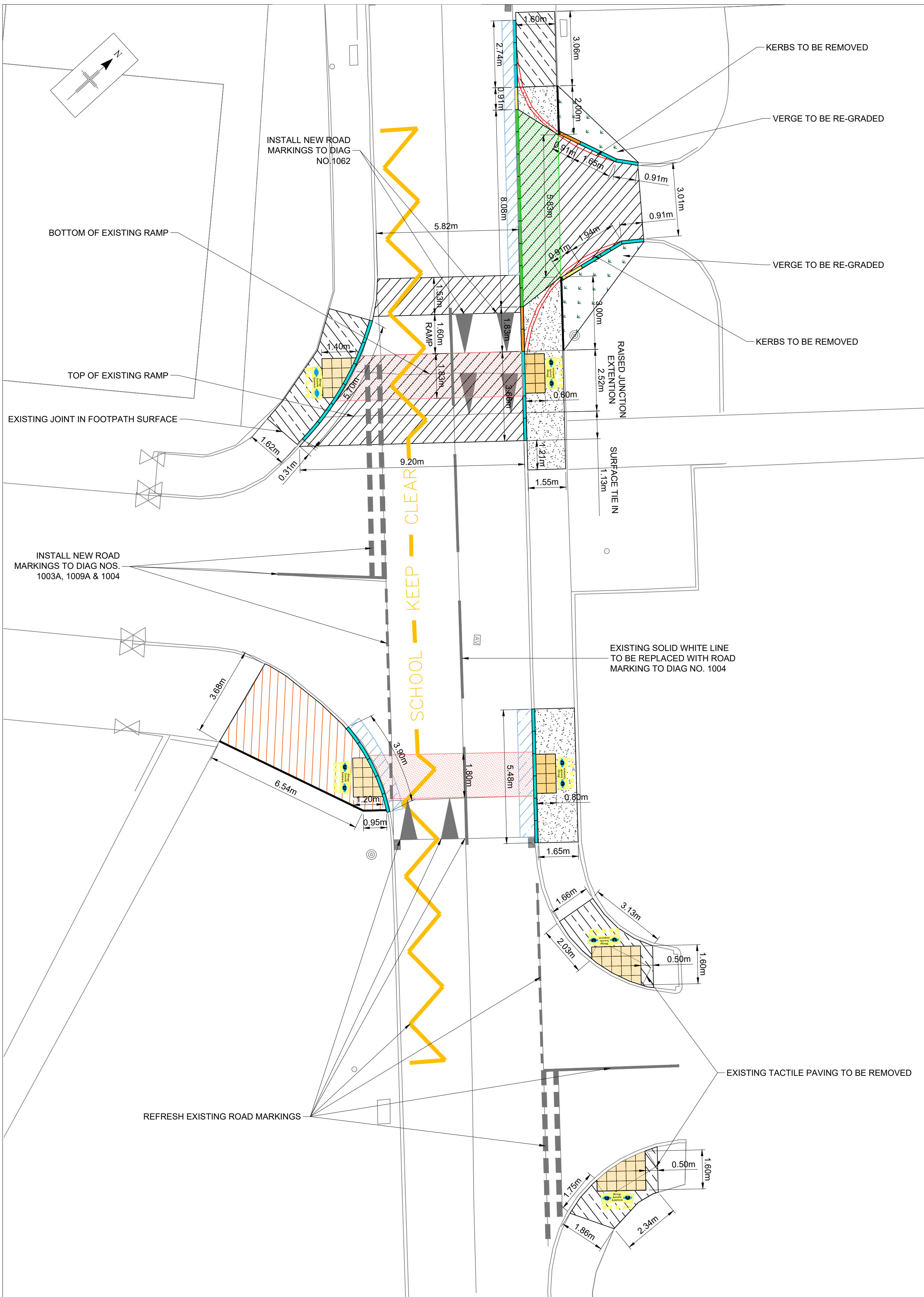
DETAIL 01 SCALE 1:100
