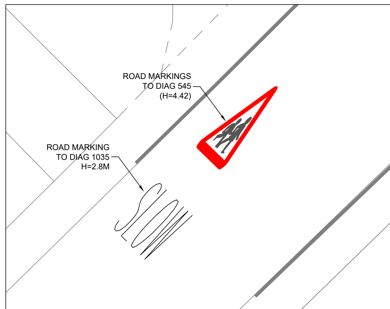
DETAIL 02 SCALE 1:100
