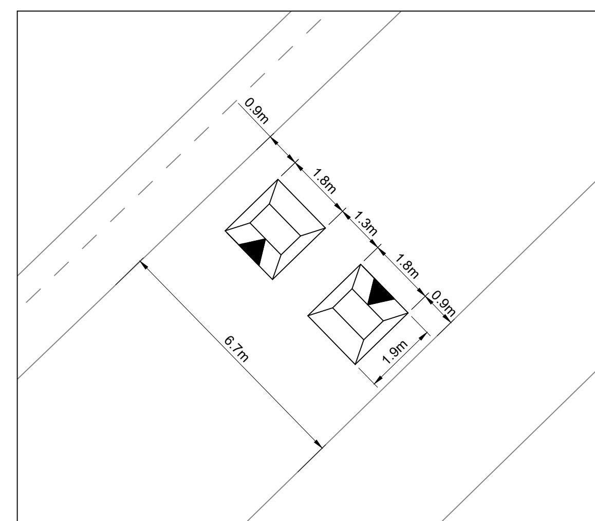
DETAIL 05 SCALE 1:100
