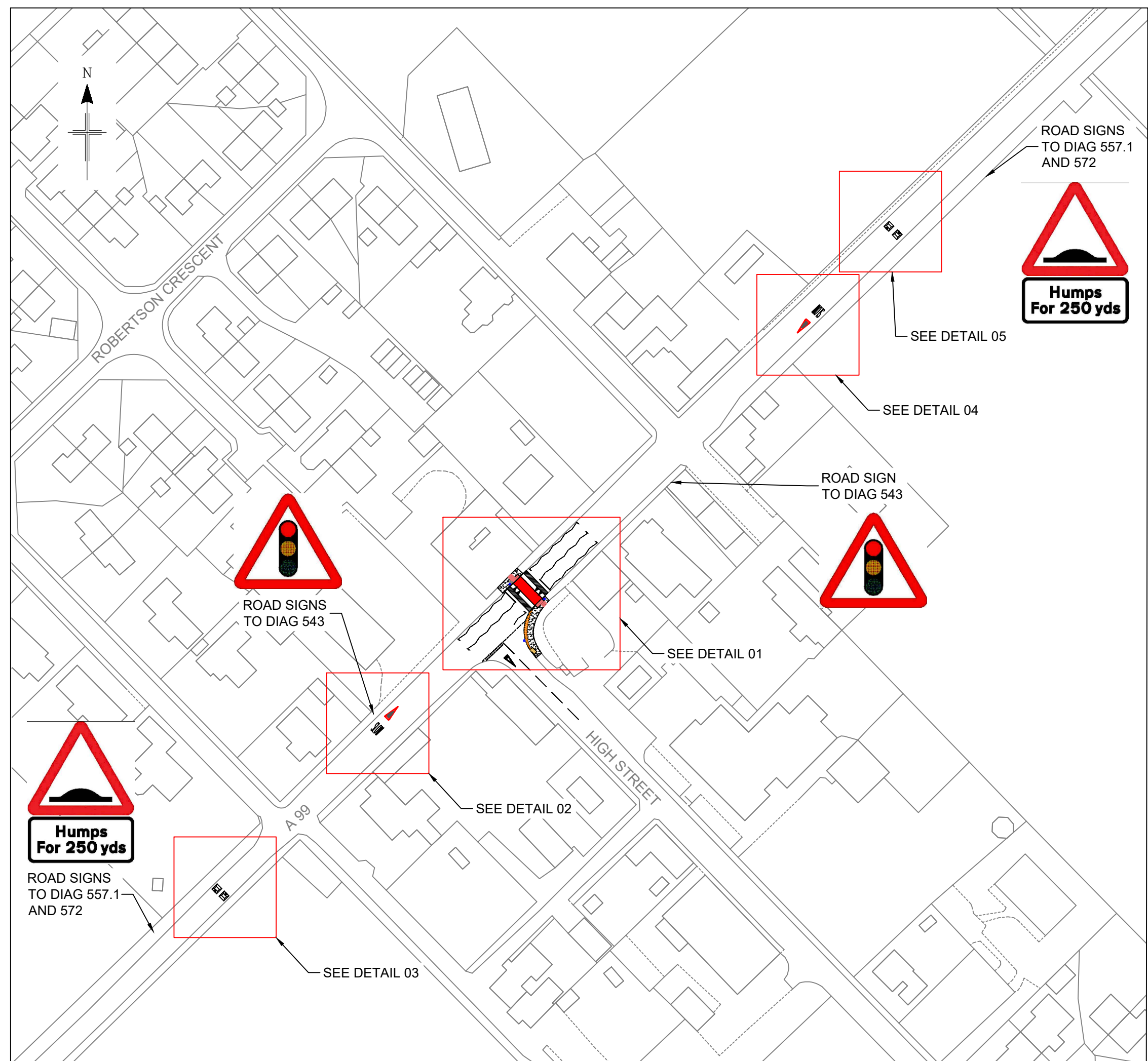
GENERAL LAYOUT SCALE 1:500
