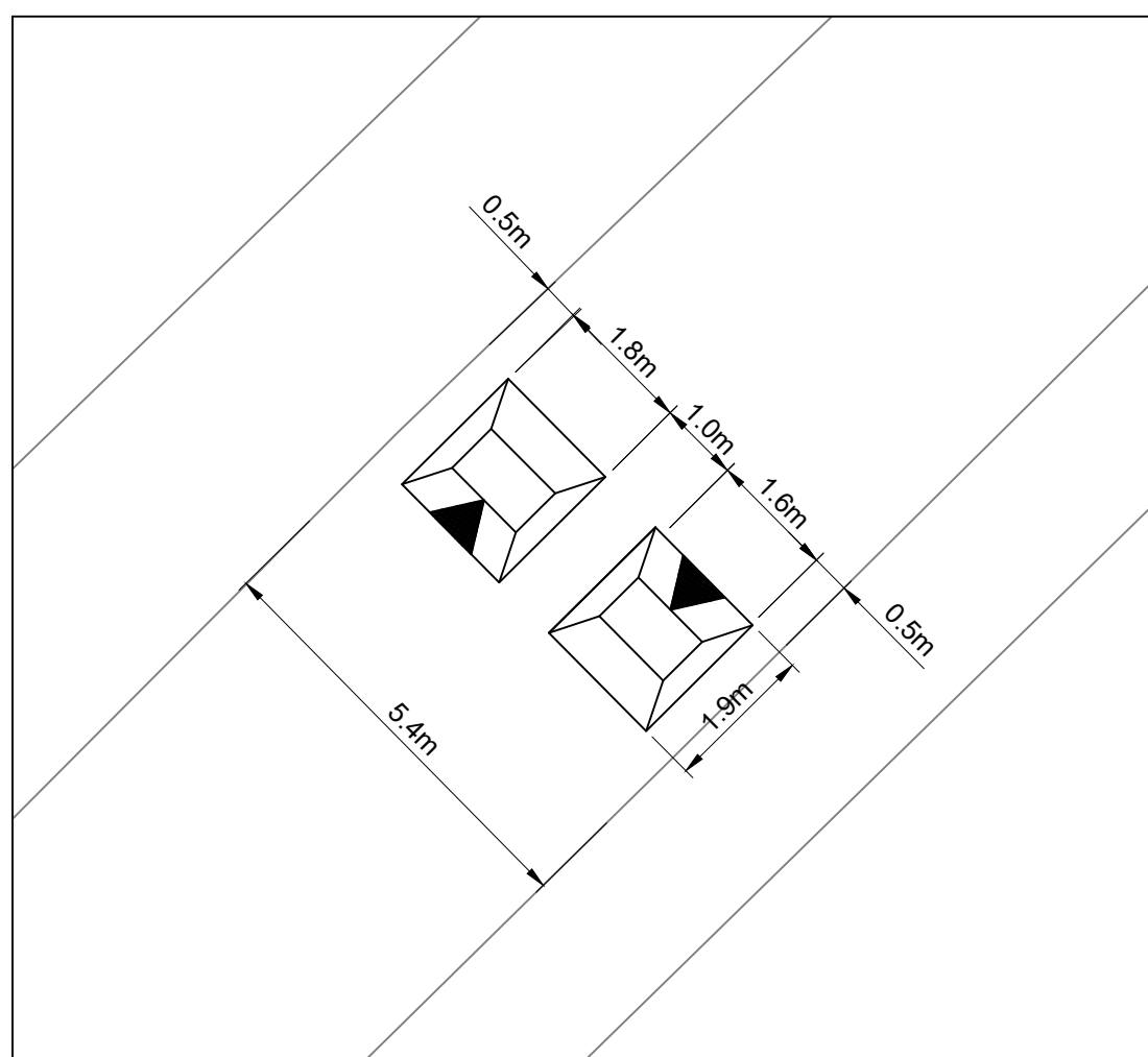
DETAIL 03 SCALE 1:100
