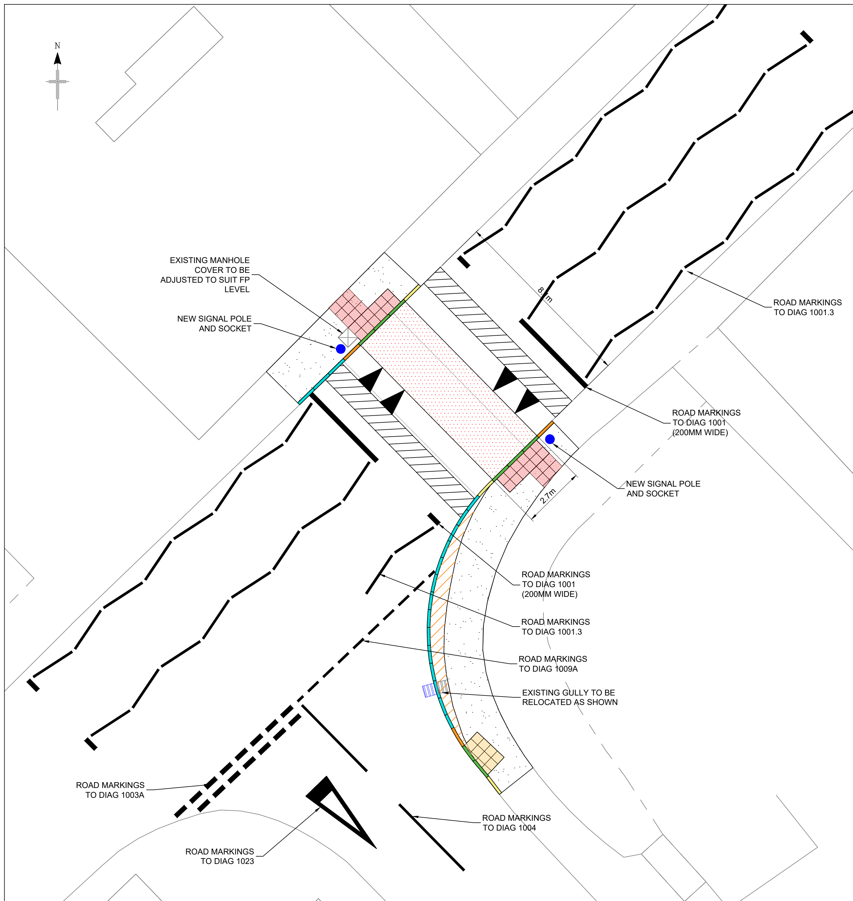
DETAIL 01 SCALE 1:100
