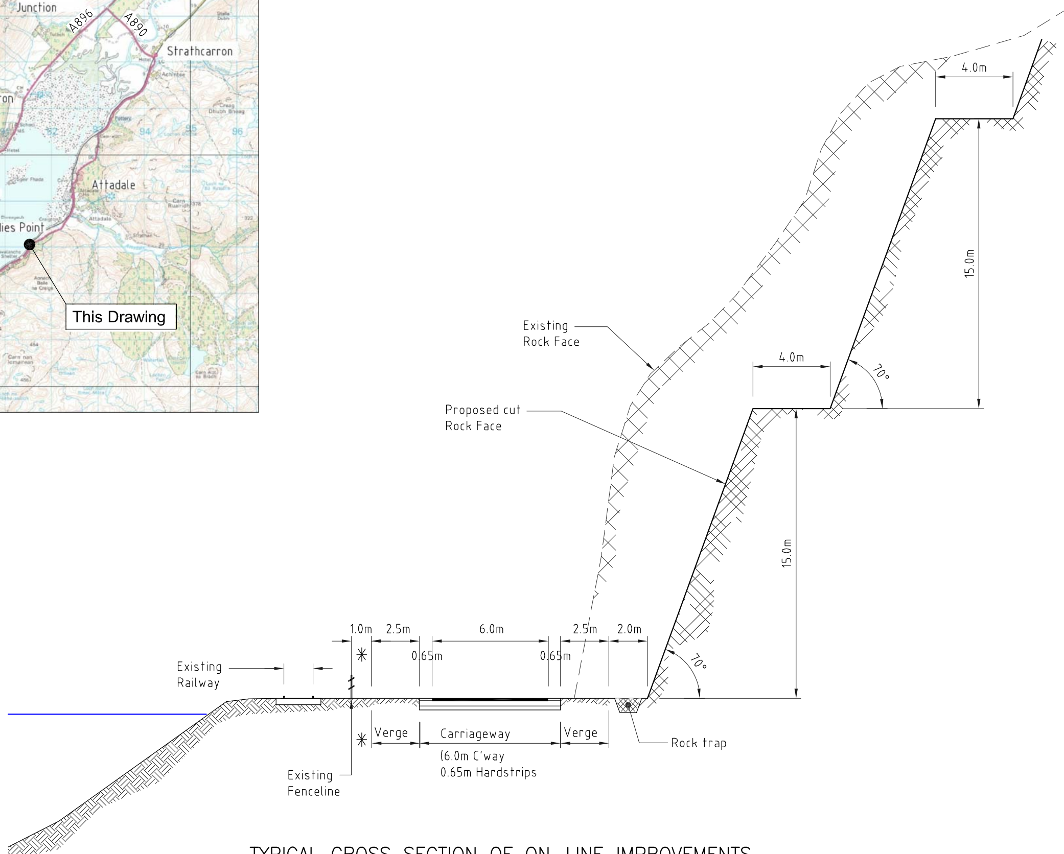
TYPICAL CROSS SECTION OF ON-LINE IMPROVEMENTS
