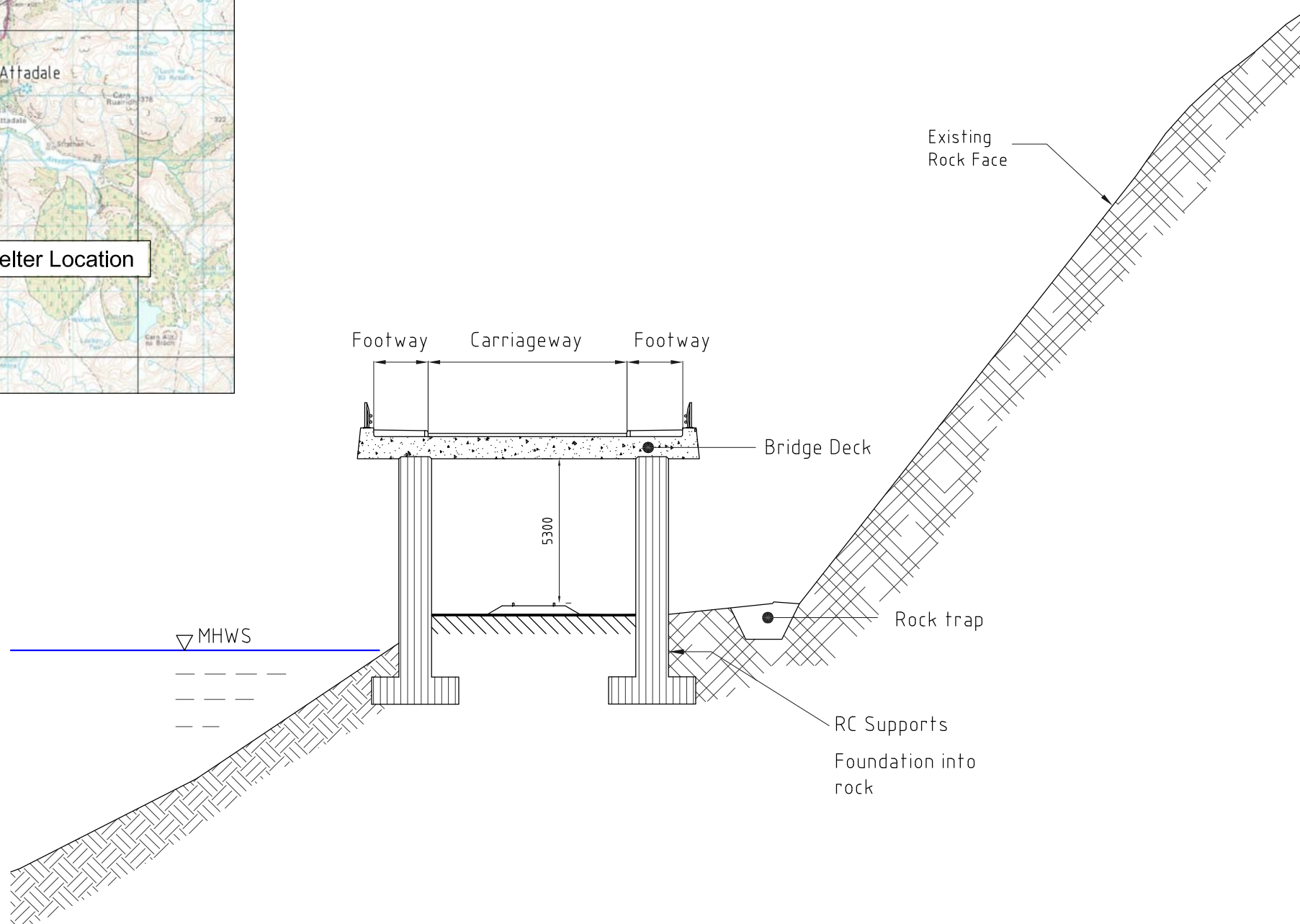
PROPOSED DETAIL EXTENDED AVALANCHE SHELTER – ALTERNATIVE A
