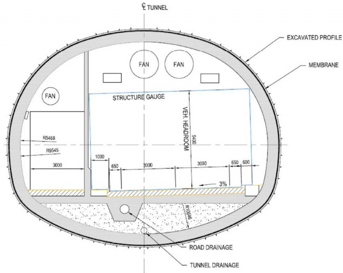
Proposed Tunnel @ Strome Narrows (Tunnel profile with undrained lining) (Not to scale)
