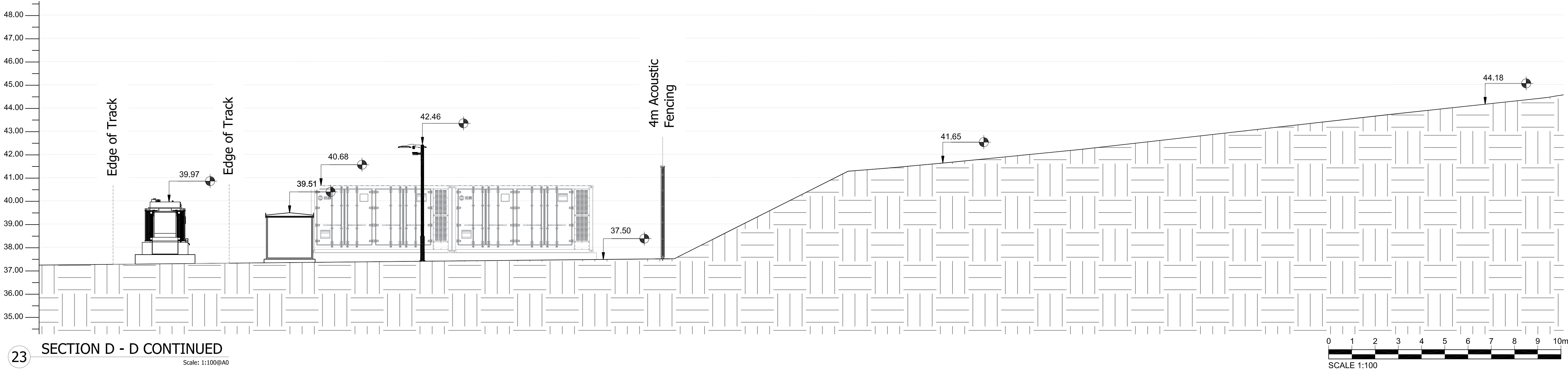
22 SECTION D - D CONTINUED Scale: 1:100(8/40)
