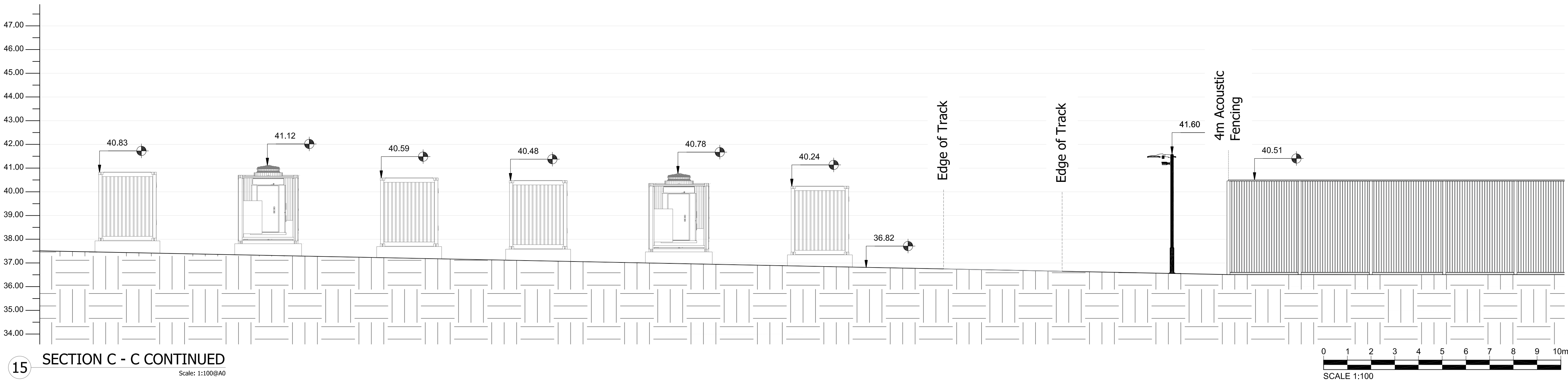
14 SECTION C - C CONTINUED Scale: 1:100(8A0)
