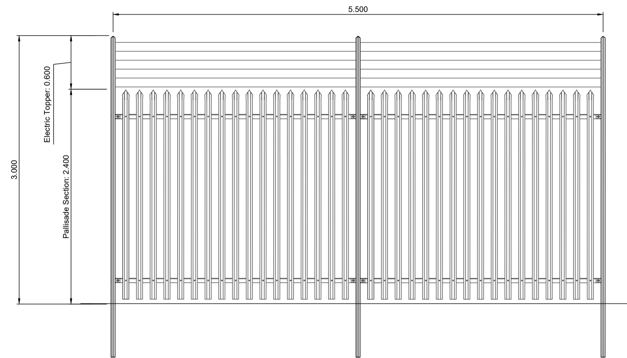
4 Typical Palisade Fence Elevation Scale 1:25 @ A1
