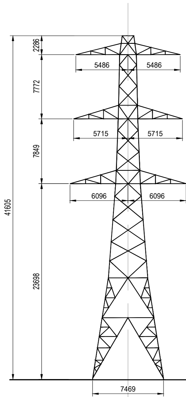
L2 D SUSPENSION TOWER
