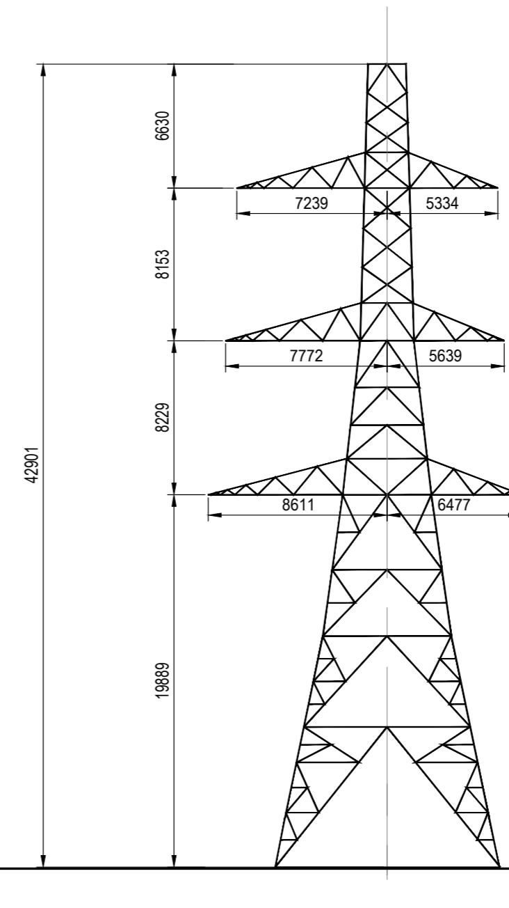
L2 D60 TENSION TOWER
