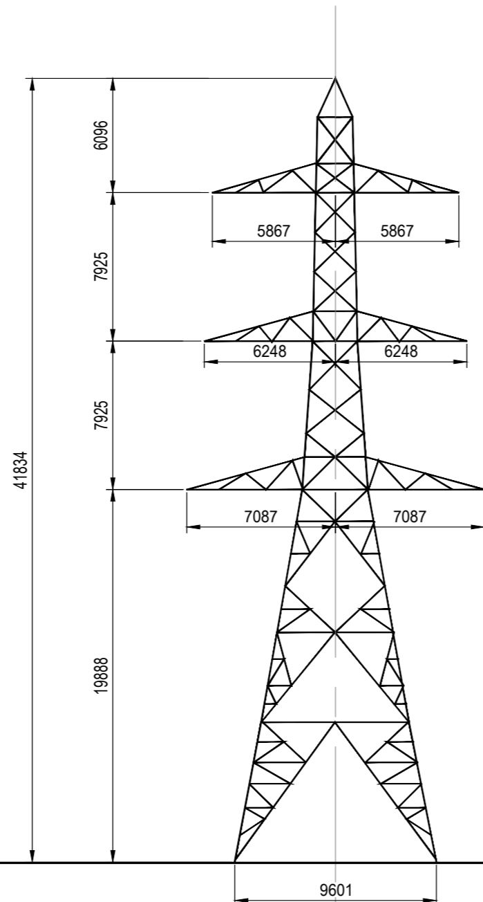
L2 D30 TENSION TOWER
