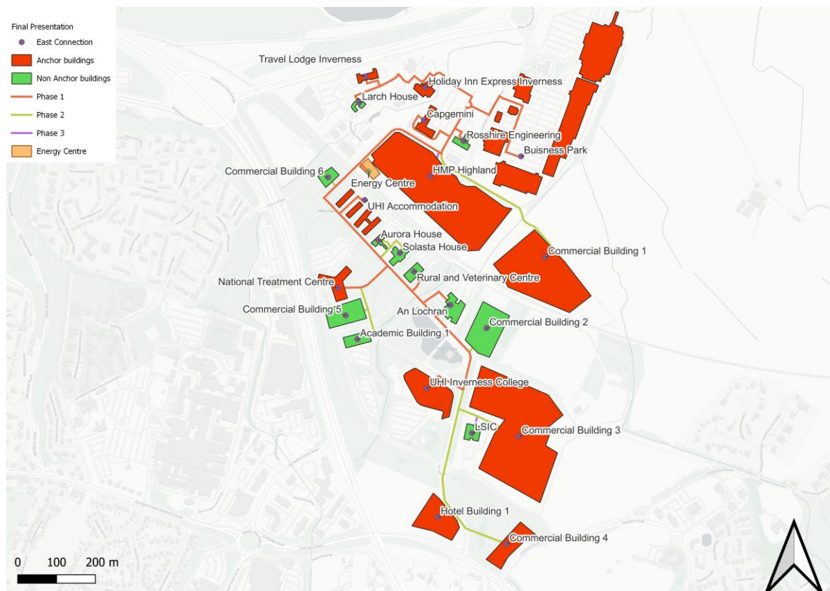
Figure 4—15 Raigmore East network overview
