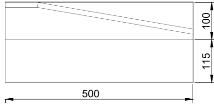
Front Elevation (LH unit)
