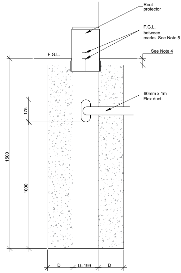
10m column
