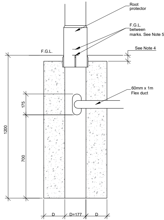
8m column
