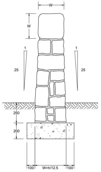
Random rubble uncoursed masonry wall with stone-on-edge cope
