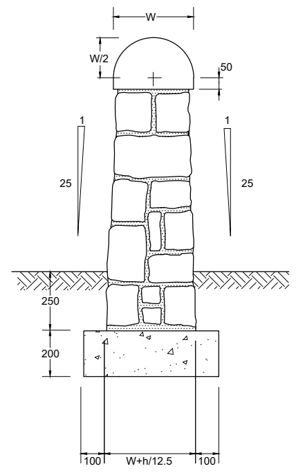
Random rubble uncoursed masonry wall with half circle dressed masonry cope
