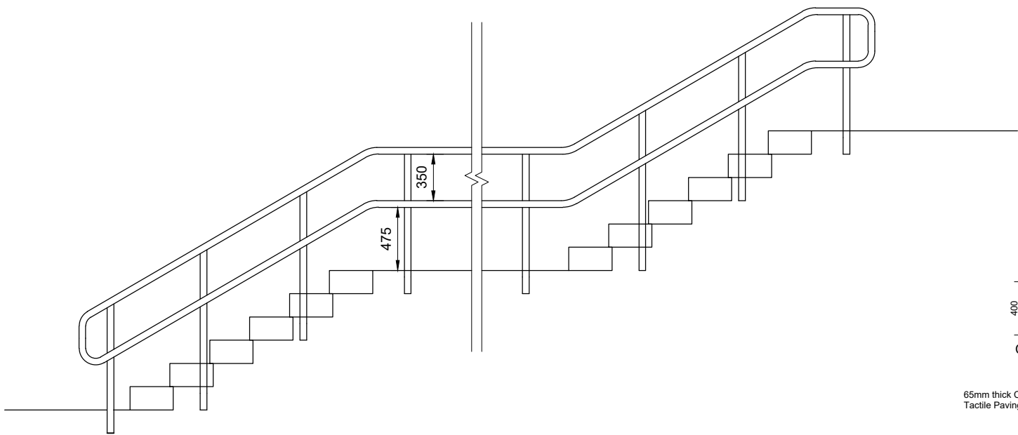
Handrails Details Not to Scale
