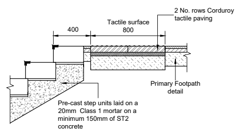
Step and tactile paving detail at Top of steps NTS
