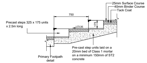
Step Detail NTS
