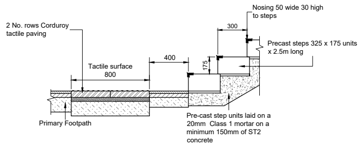
Step and tactile paving detail at Bottom of Steps NTS
