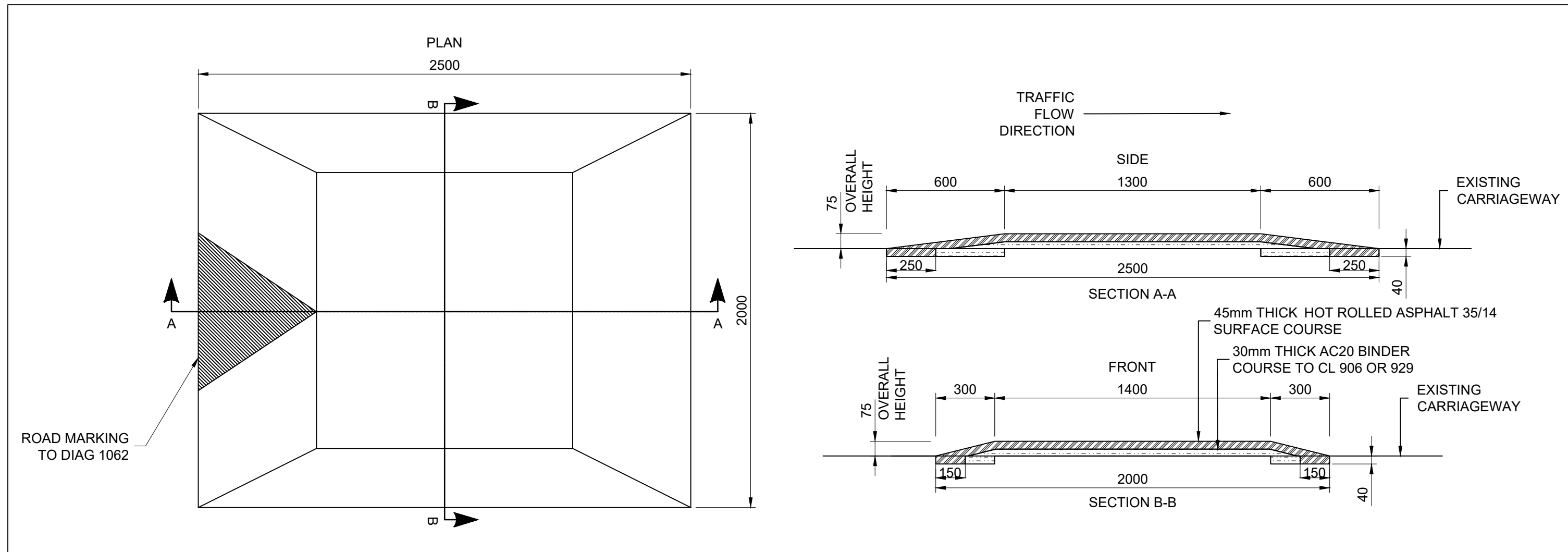
DETAIL 02 SCALE 1:20
