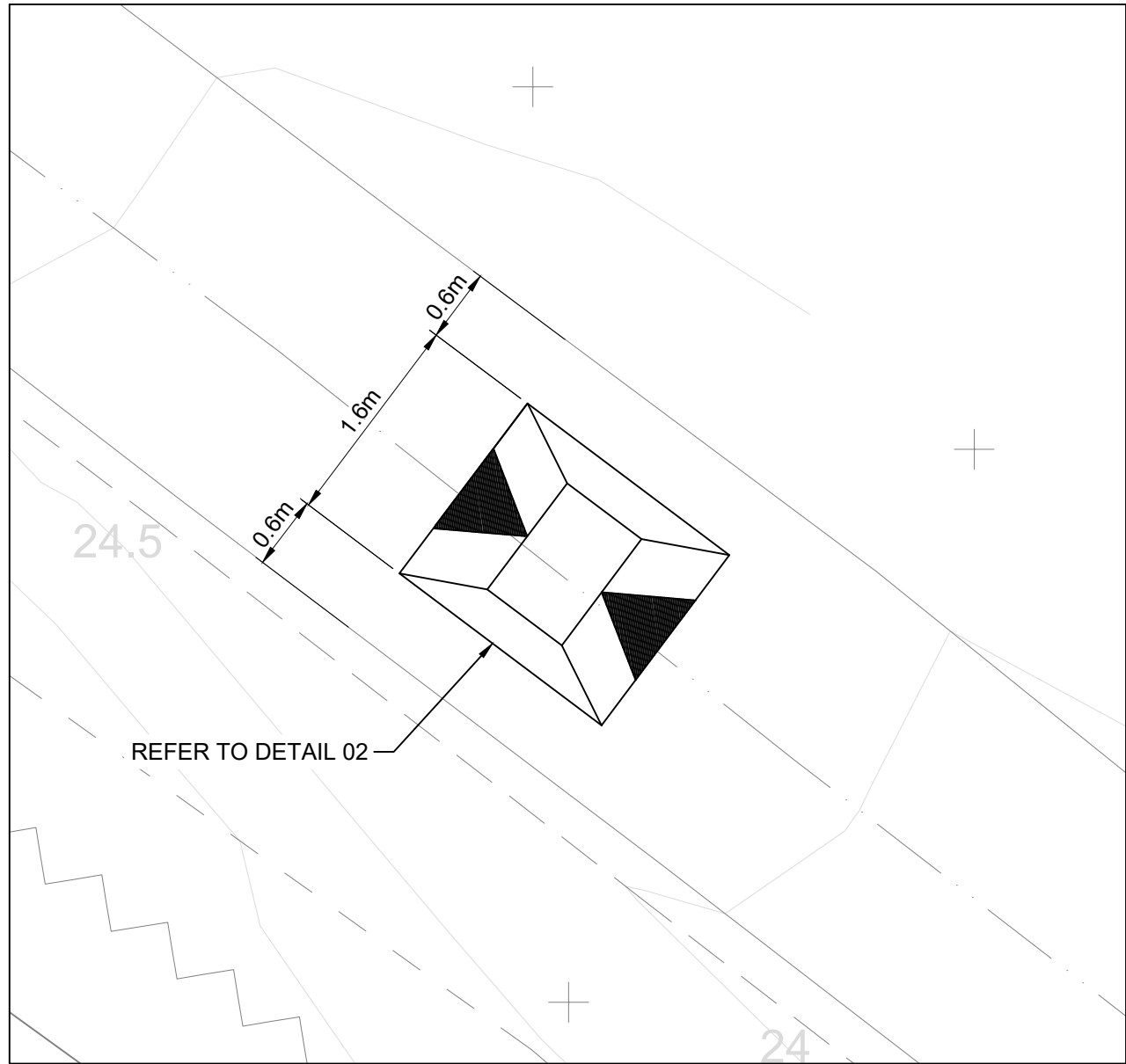
DETAIL 01 SCALE 1:100
