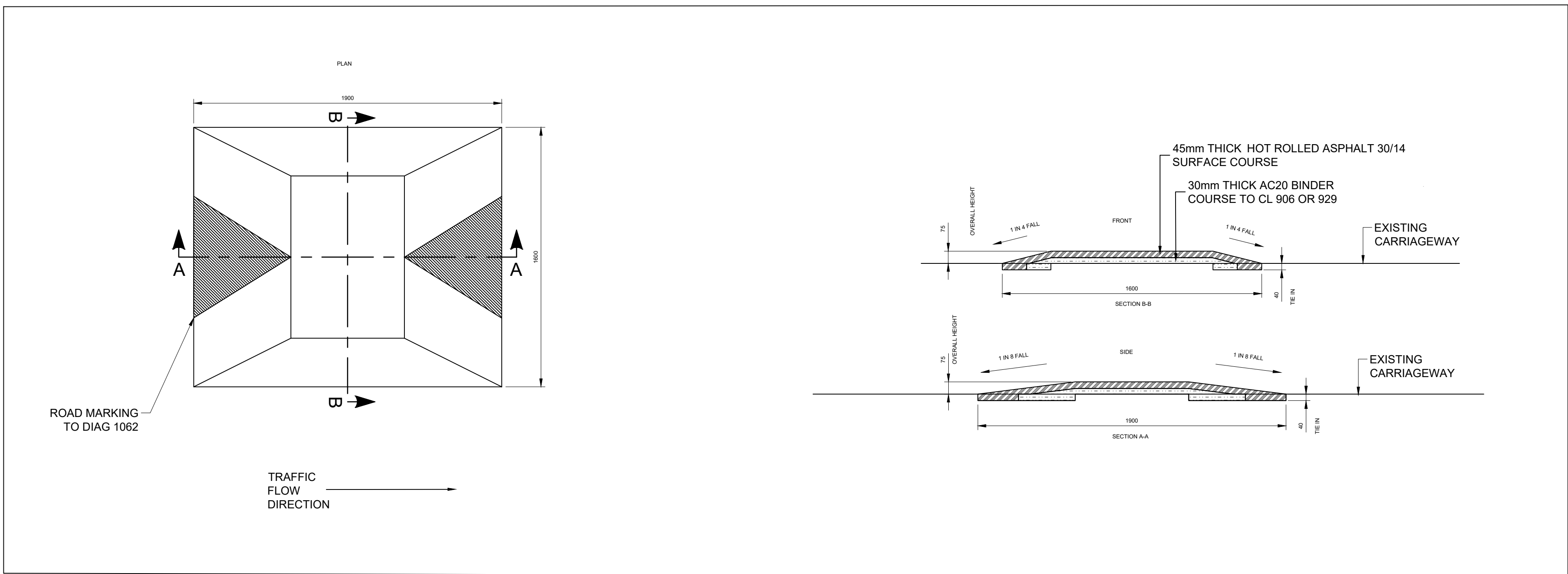
DETAIL 02 SCALE 1:100
