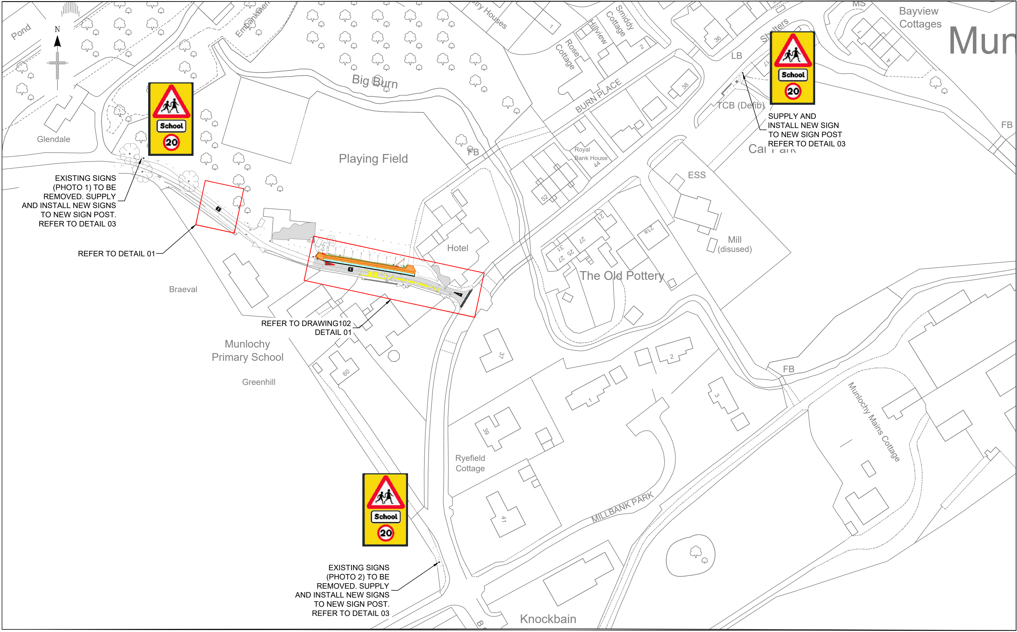
GENERAL LAYOUT SCALE 1:1000
